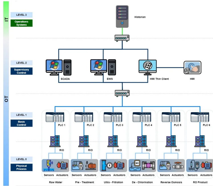
Figure 2: Reference network architecture for Secure Water Treatment (SWaT) Testbed [5]
